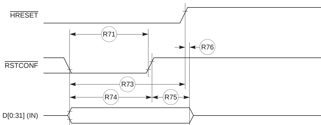
Figure 36. Reset Timing – Configuration from Data Bus
